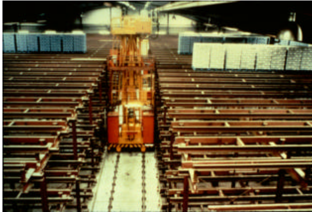
Figure 14.60. Two-Sided Deep Lane Storage Warehouse
