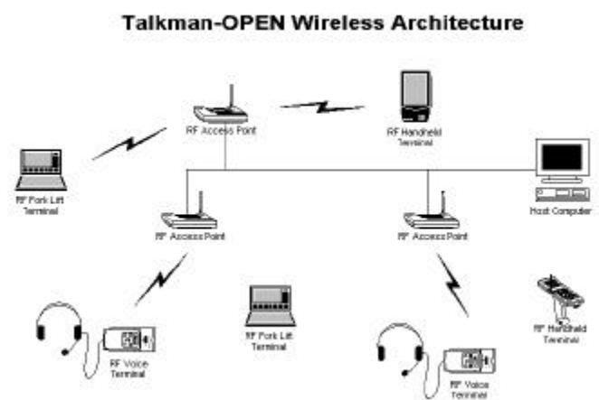
Figure 14.51. Radio-Frequency Terminal Architecture for Warehouse Communications (Figure courtesy of Vocollect)
