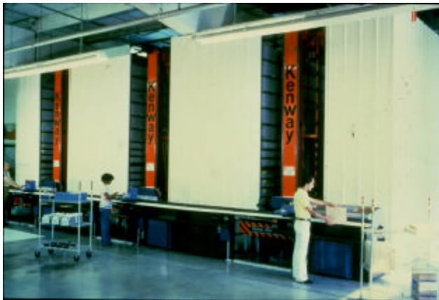
Figure 14.57. Miniload Automated Storage/Retrieval System
