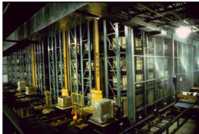
Figure 14.53. Unit Load Automated Storage/Retrieval System
