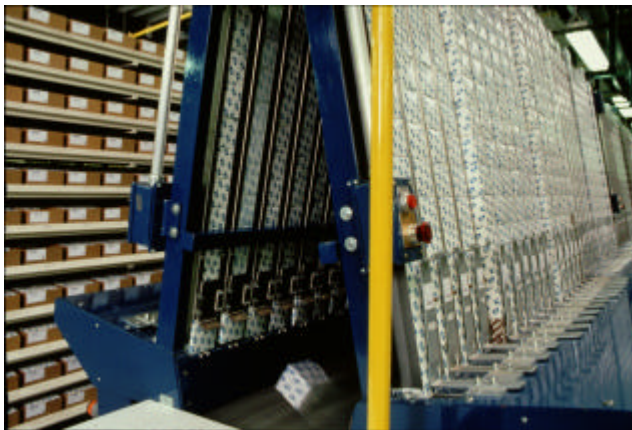
Figure 14.11. Automatic Order Picking A-Frame with Take-Away Belt Conveyor (Picture courtesy of Electrocom)
