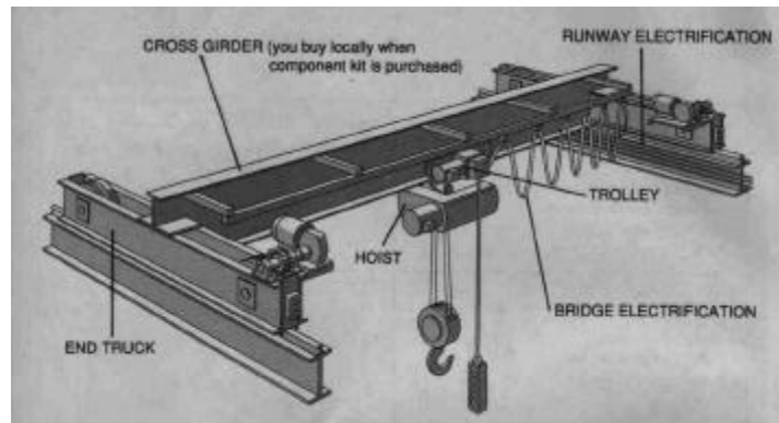
Figure 14.19. Bridge Crane
