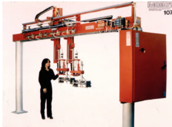
Figure 14.20. Bridge Crane for Jet Engine Assembly
