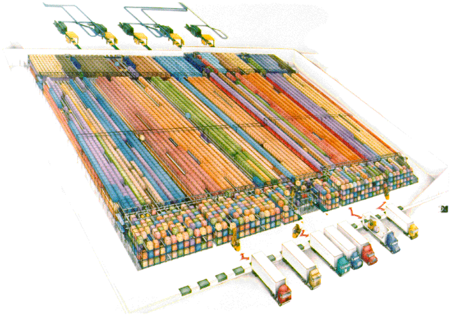
Figure 62. Deep Lane Unit Load Staging Warehouse (Activ System, photo courtesy of Retrotech)
