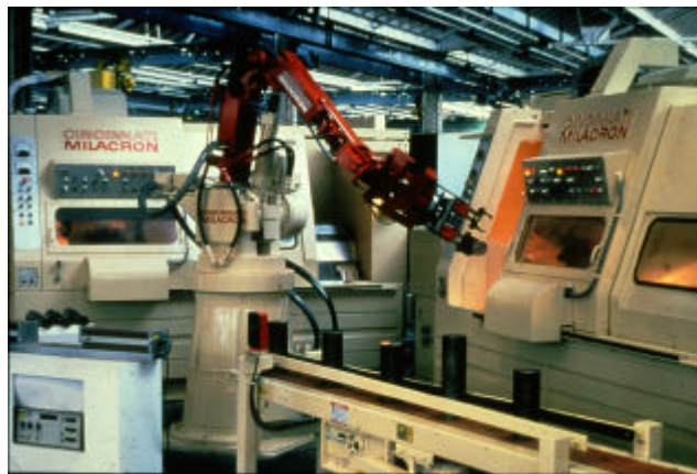
Figure 14.70. Robotic Part Loading in an Automated Machining Cell
