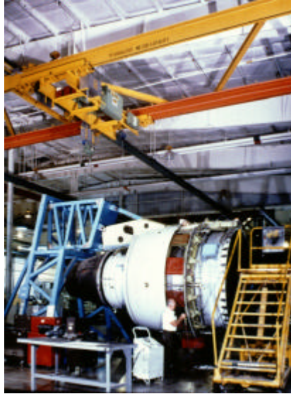
Figure 14.20. Bridge Crane for Jet Engine Assembly
